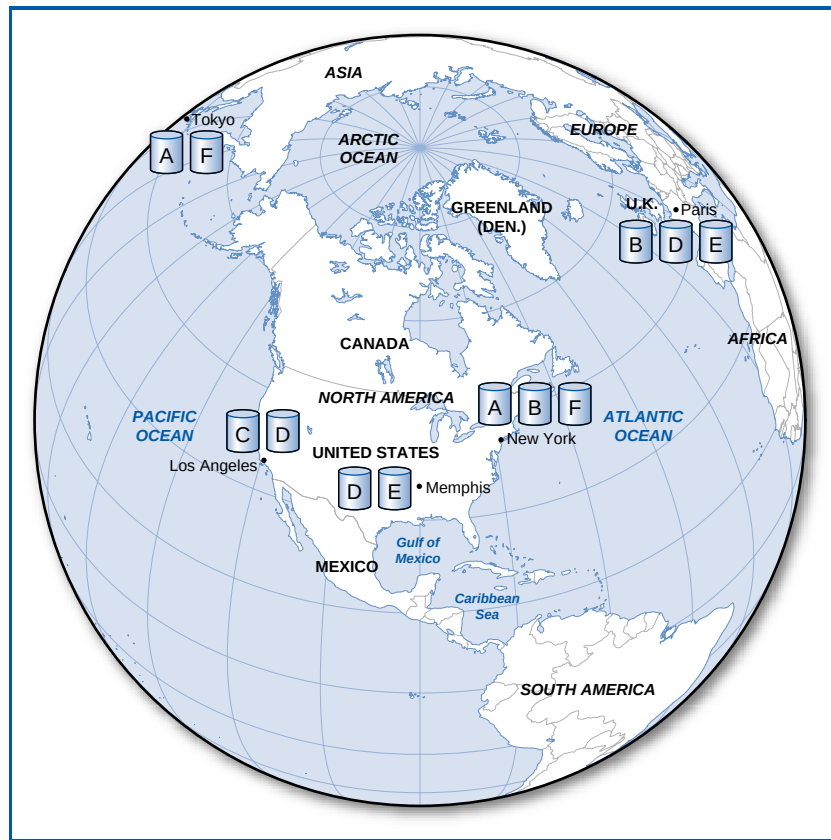
FIGURE 12.9 Distributed database with targeted data replication
